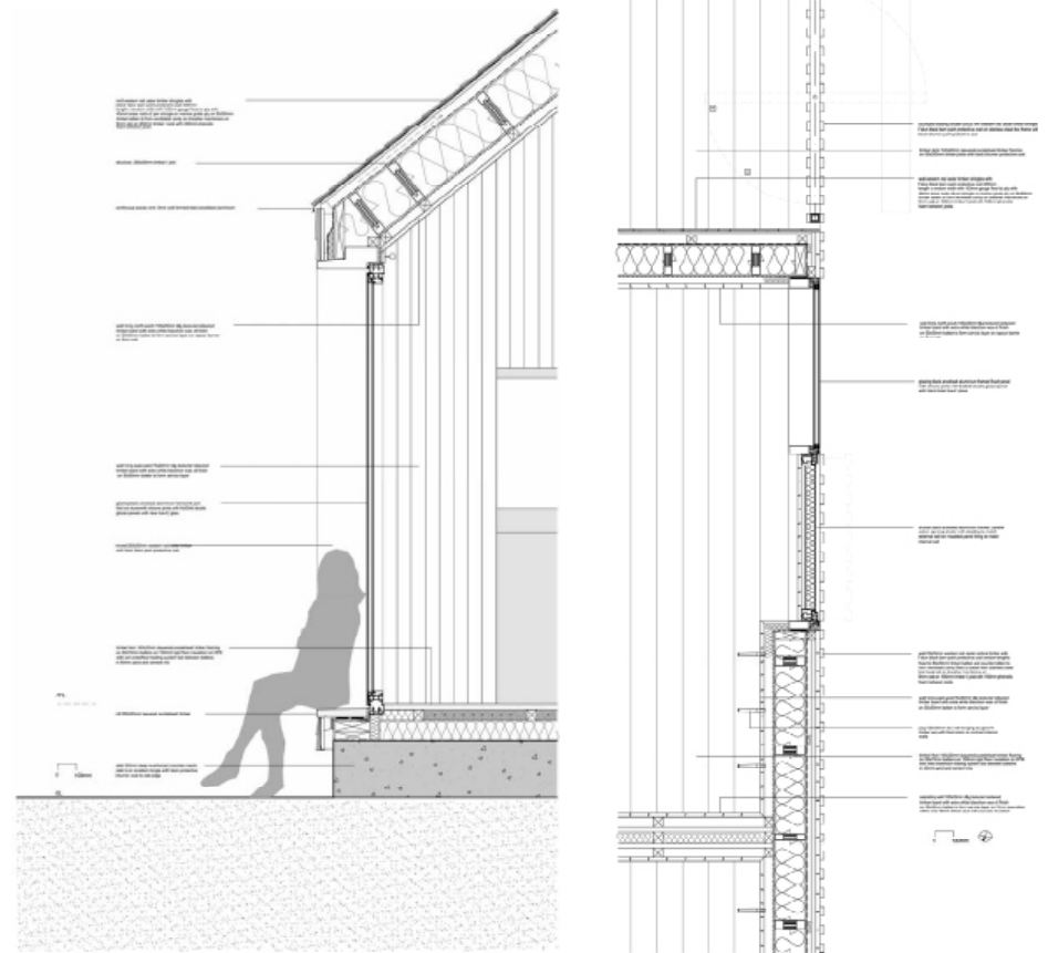
Detail Sections - As Built
