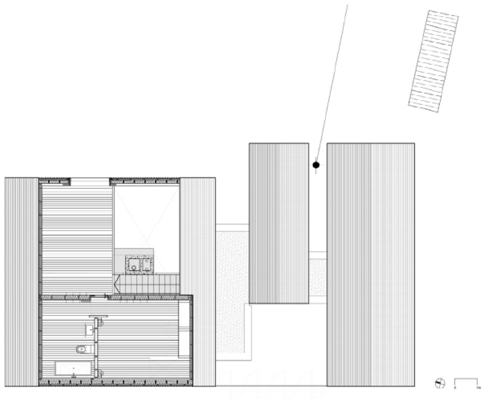
First Floor Plan Drawing - As Built
