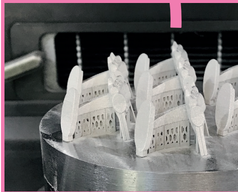
3D platinum printing
