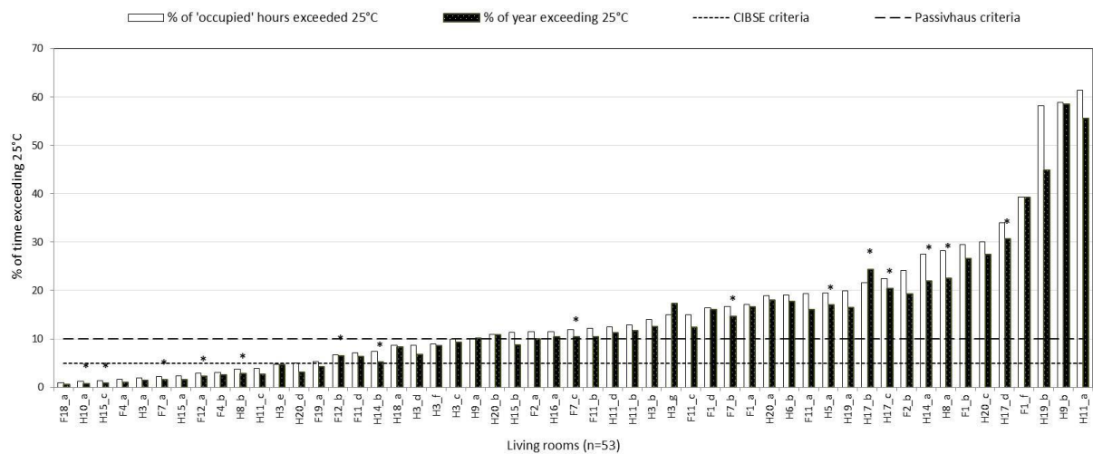
Figure 2. a) Percentage of time the temperature exceeded 25°C in bedrooms; and (b) percentage of time the temperature exceeded 25°C in living rooms.
