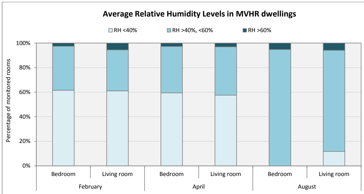
Figure 4.2g. Average relative humidity levels in dwellings with MVHR
