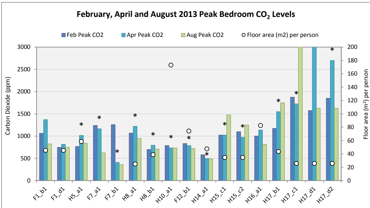
Figure 4.1f. Peak bedroom CO 2 levels in dwellings with MVHR * Passivhaus dwellings
