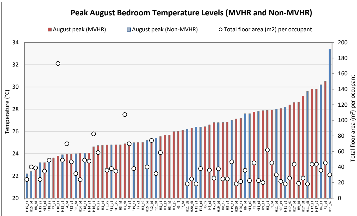
Figure 8.4f. Peak August bedroom temperatures in MVHR and Non MVHR homes
