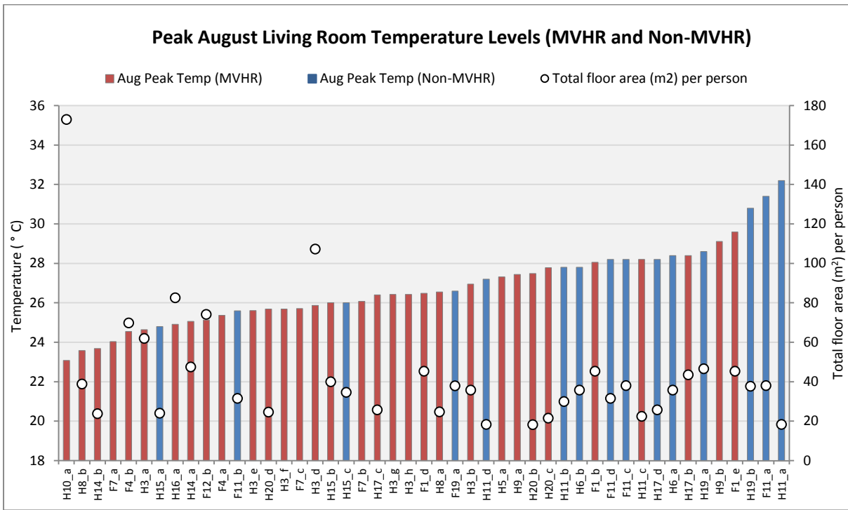
Figure 8.4e. Peak August living room temperatures in MVHR and Non MVHR homes
