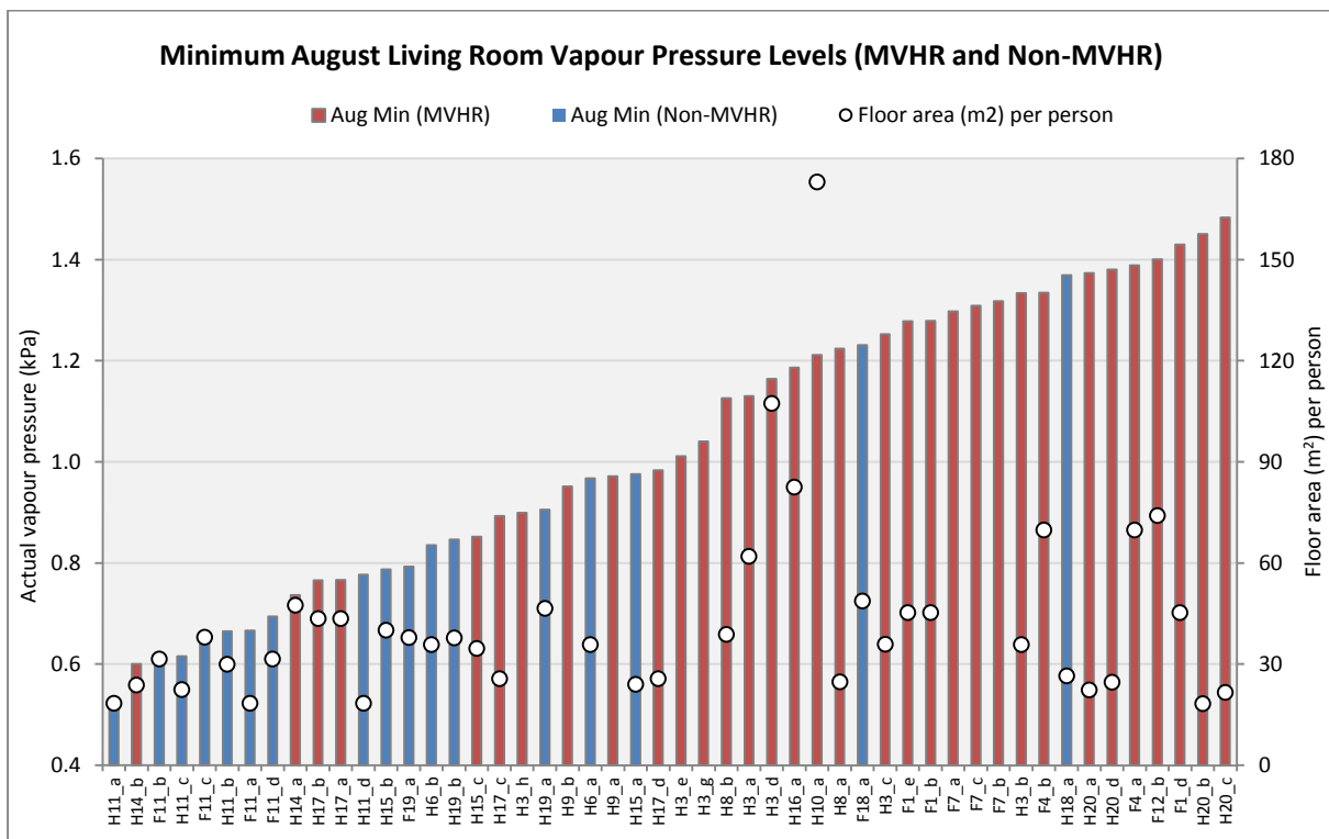
Figure 8.5d. Minimum August living room vapour pressure levels in MVHR and Non MVHR homes
