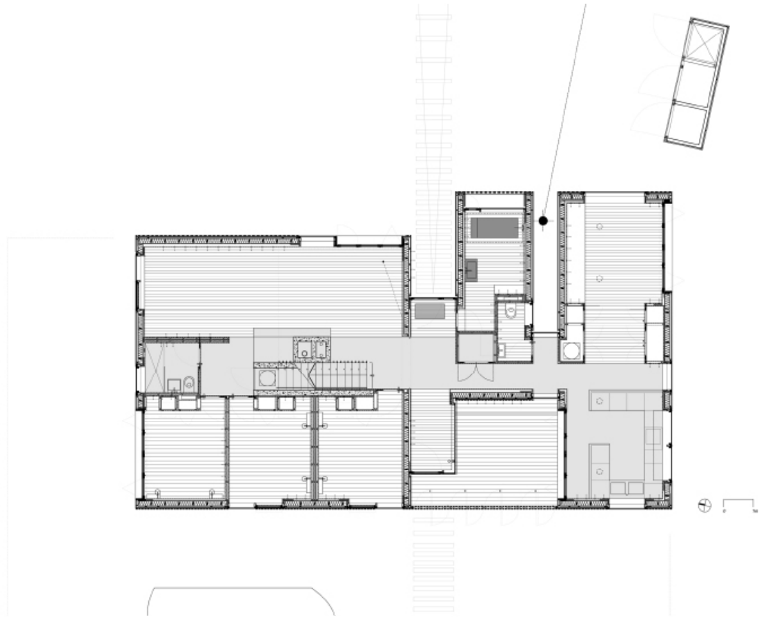
Ground Floor Plan Drawing - As Built
